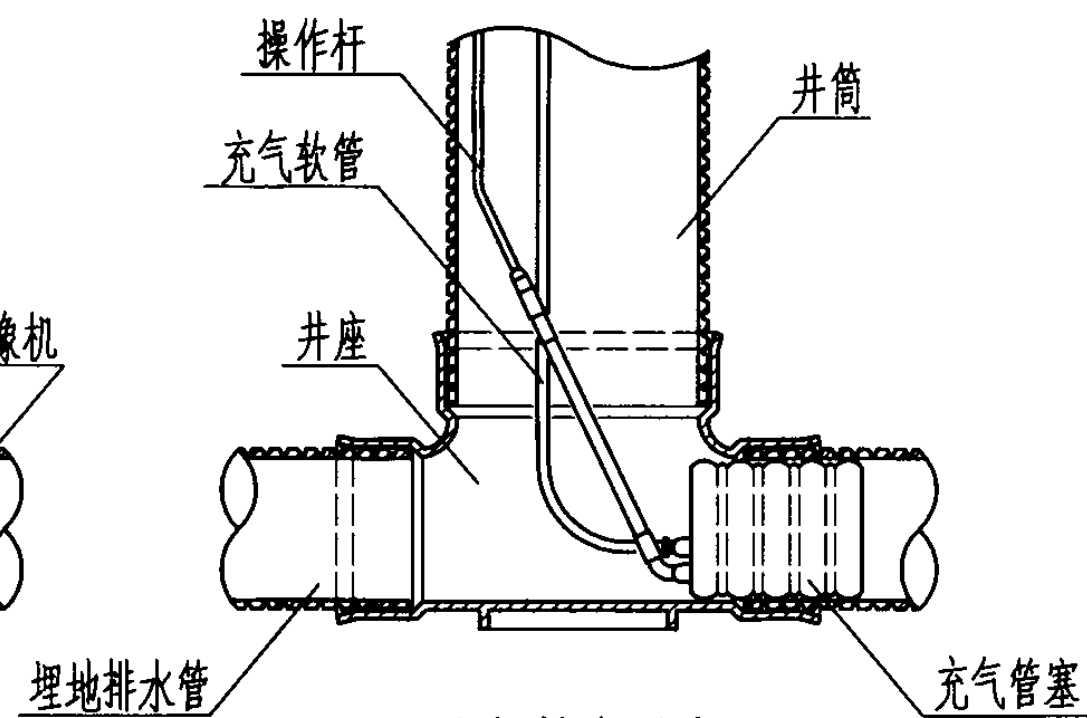
充气管塞封堵
