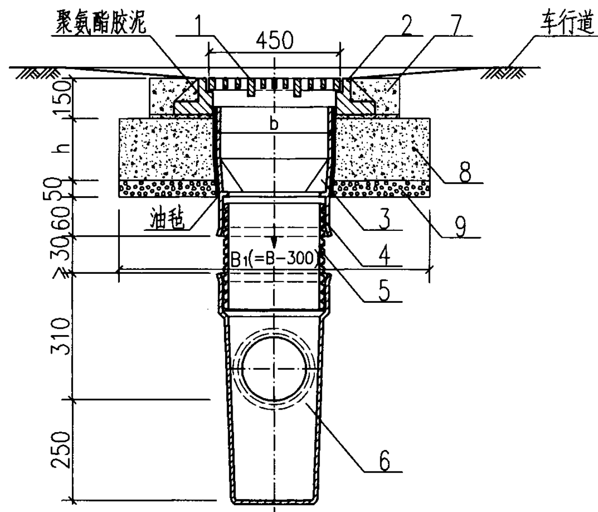
2-2
