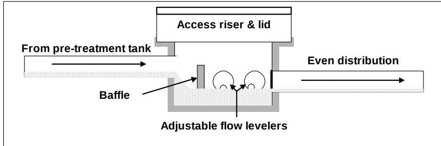
Figure 11-1: Distribution box
